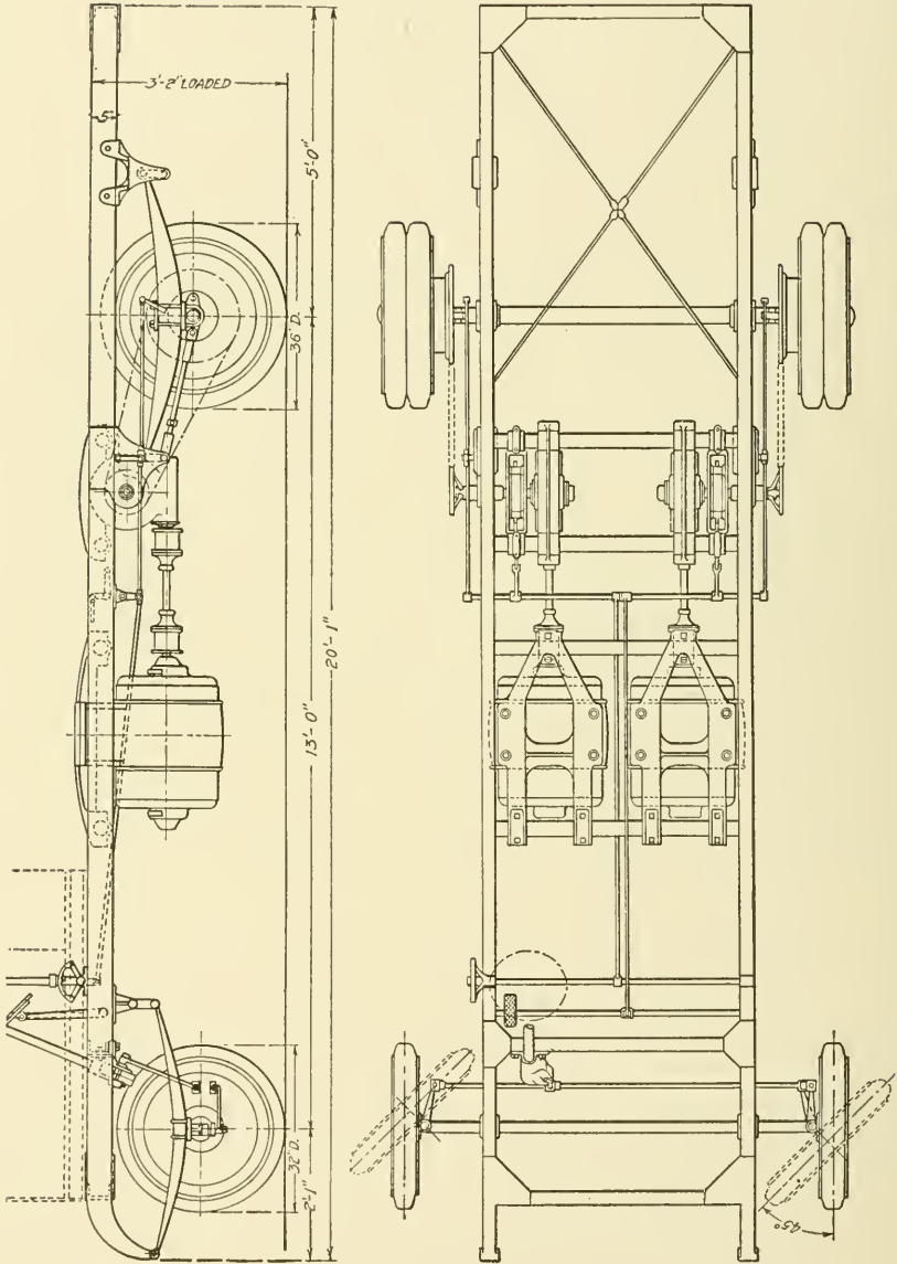
Figs. 19 and 20. Elevation and Plan of Leeds Chassis Showing Motor Gearing and Steering Construction
